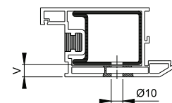
profilo in PVC
